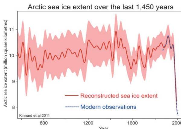
Figure2: Change in Arctic sea ice extent, Kinnard et al (2011)
